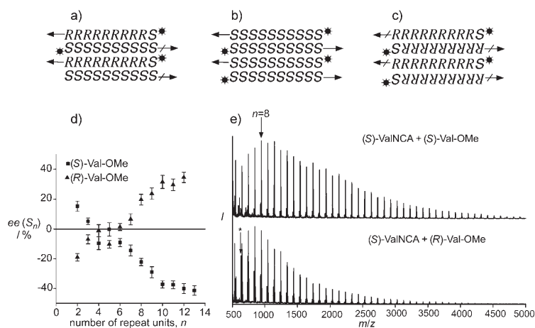
Figure 3. a–c) Different types of ap \beta sheets comprising four strands of homochiral sequences with a S^* repeat unit of the initiator attached at the C terminus:
